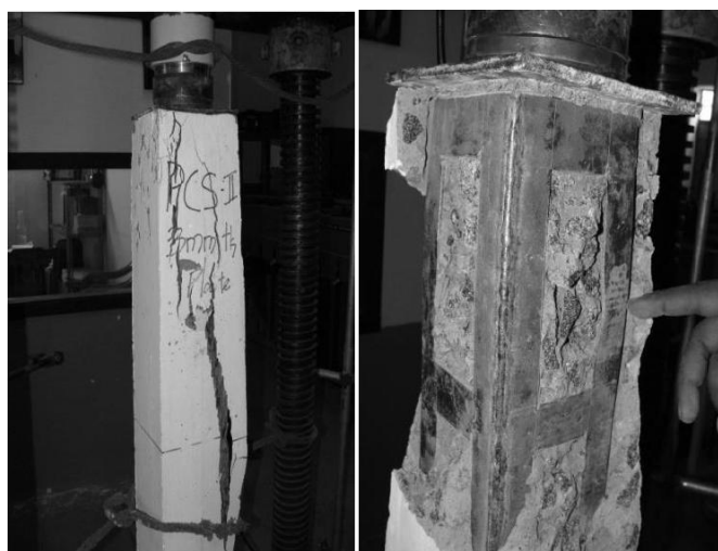
Fig.6. S4P21 and S4P22 Specimens
