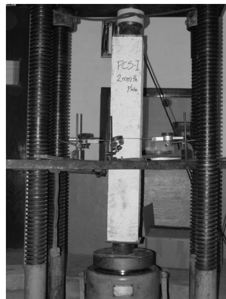
Fig.4. Experimental Setup
