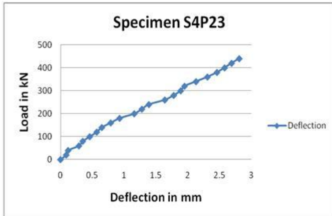
Fig.7. Load-Displacement Curve for Specimens
